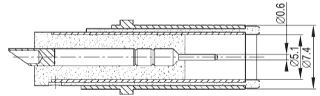
MATING PLUG
