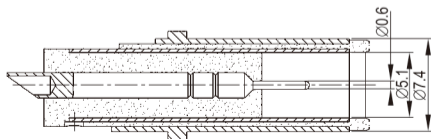
MATING PLUG
