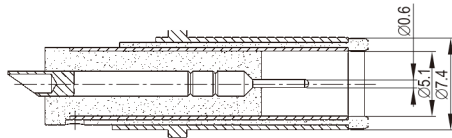
MATING PLUG
