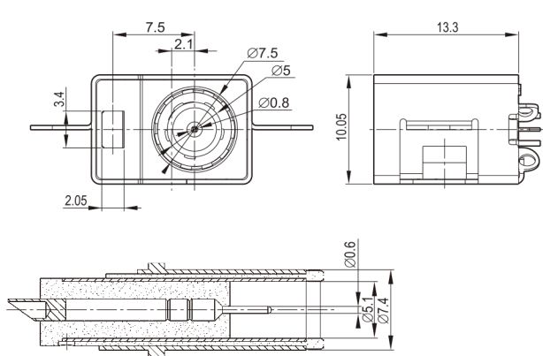
MATING PLUG
