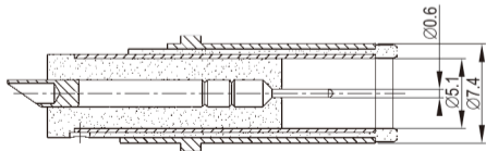
MATING PLUG
